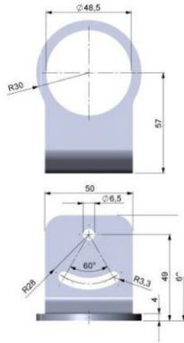
Mounting bracket (fixed) for IR20 laser
